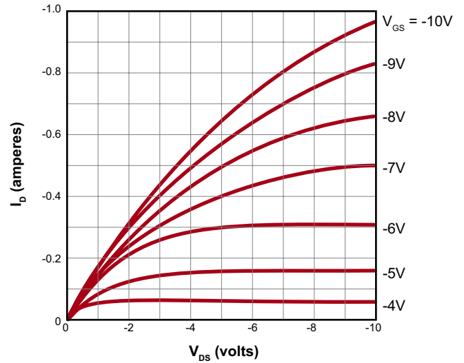
Saturation Characteristics
