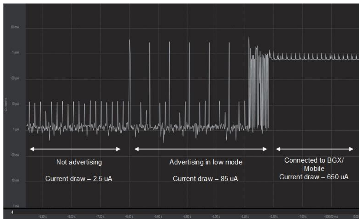
Figure 4.3. Energy Profiler Capture of BGX with 9600 bps UART Baud Rate
