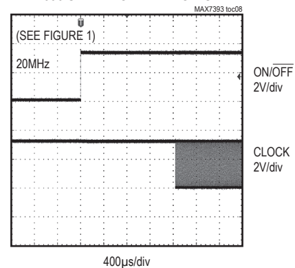
MAX7393 SETTLING TIME FROM START
