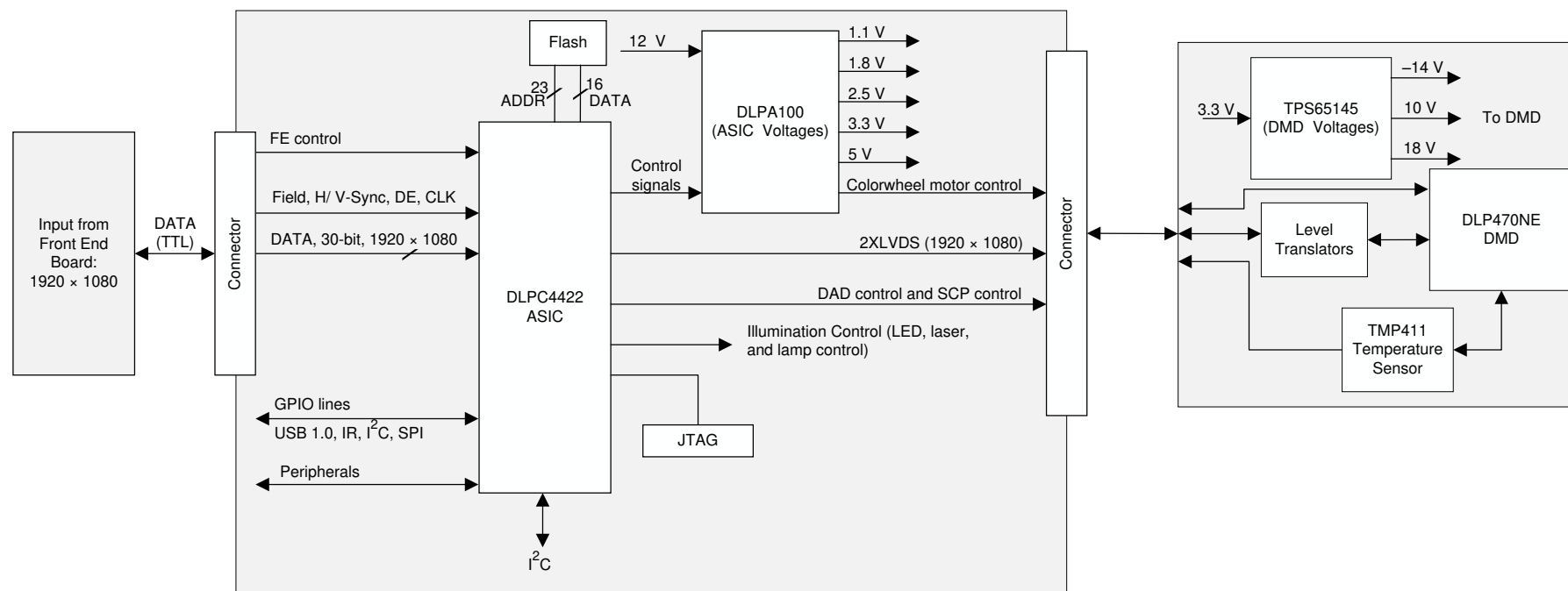
Figure 12. Typical 1080P Application Diagram
