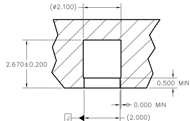
SECTION G-G DATUM J SCALE 16/1
