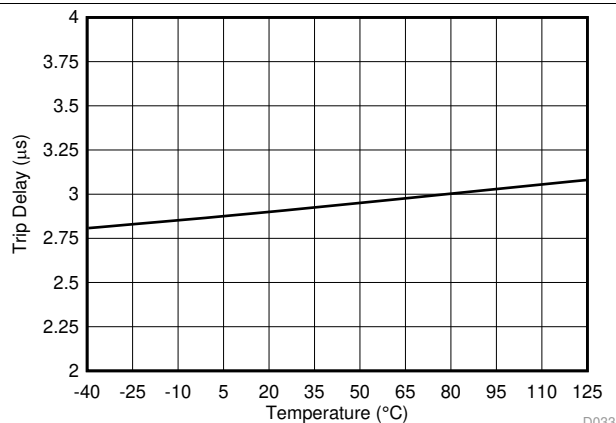
Figure 38. \overline{\text{OR}} Pin Trip Delay vs Temperature
