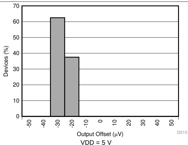
Figure 18. Shunt-Sense Amplifier Output Offset Histogram
