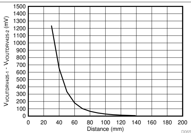
Figure 70. Difference Between Two DRV425-Q1 Outputs vs Distance to the Magnet
