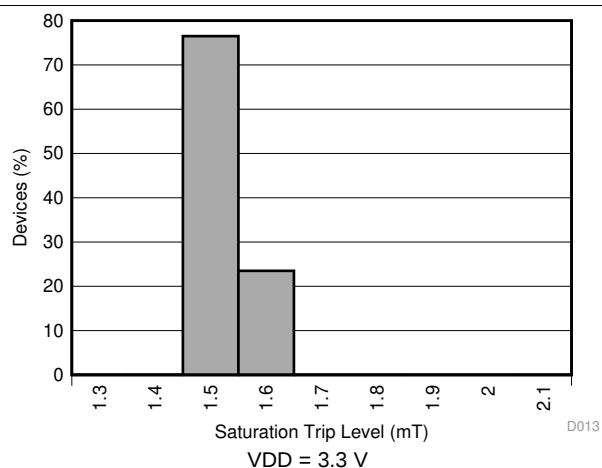
Figure 14. Fluxgate Sensor Saturation ( \overline{\text{ERROR}} Pin) Trip Level Histogram
