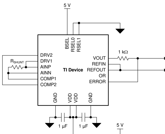
Figure 64. Field Overrange Detection Using a Combined VOUT and \overline{\text{ERROR}} Pin
