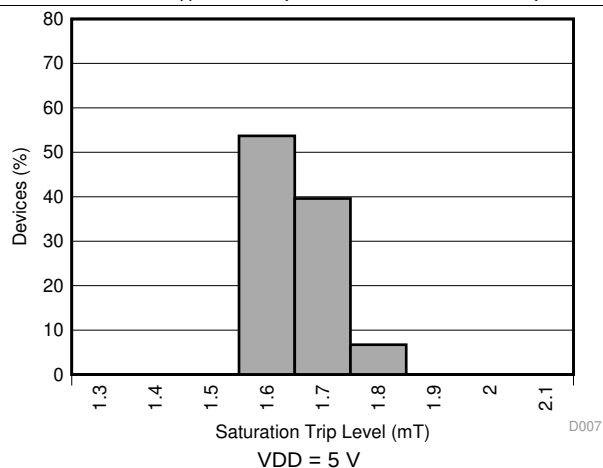
Figure 13. Fluxgate Sensor Saturation ( \overline{\text{ERROR}} Pin) Trip Level Histogram
