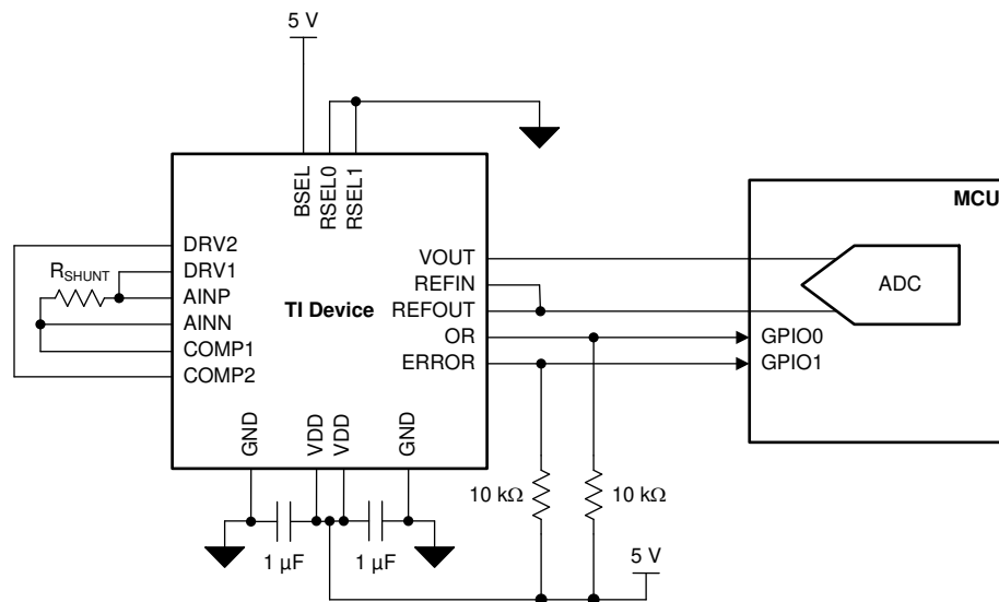
Figure 67. Linear-Position Sensing
