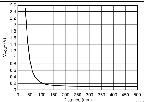
Figure 69. Analog Output Voltage of the DRV425-Q1 vs Distance to the Magnet
