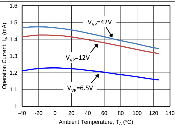
Figure 1. Operation Current vs Temperature
