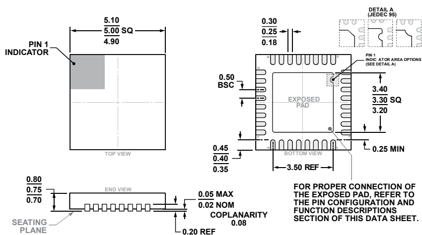
Figure 18. 32-Lead Lead Frame Chip Scale Package [LFCSP] 5 mm × 5 mm Body and 0.75 mm Package Height (CP-32-20)
