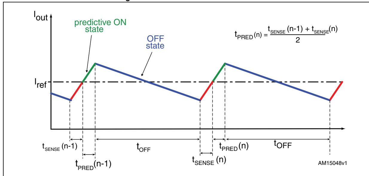
Figure 16. Predictive current control
