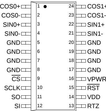
Figure 3. 33976 Pin Connections
