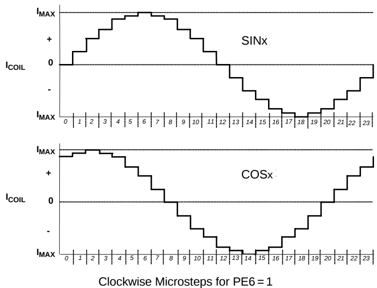
Figure 9. Clockwise Microsteps
