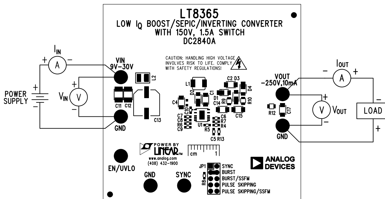
Figure 1. DC2840A Proper Equipment Setup
