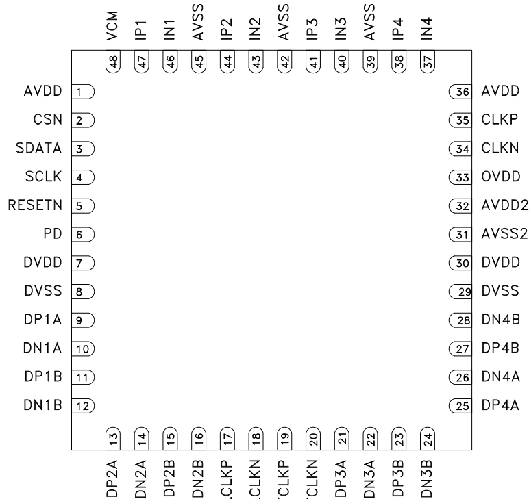
Figure 2: Package diagram
