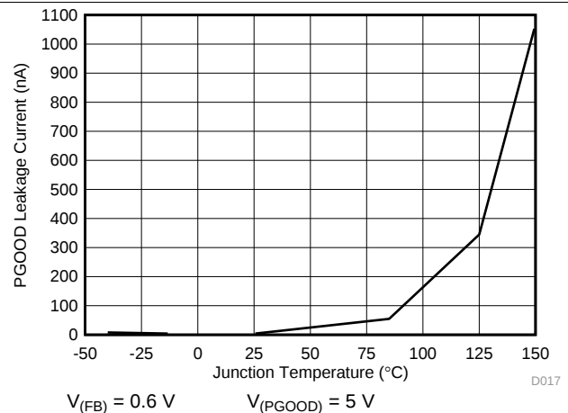
Figure 20. PGOOD Leakage Current vs Junction Temperature
