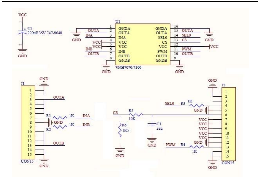
Figure 1. VN7070BAS evaluation board schematic
