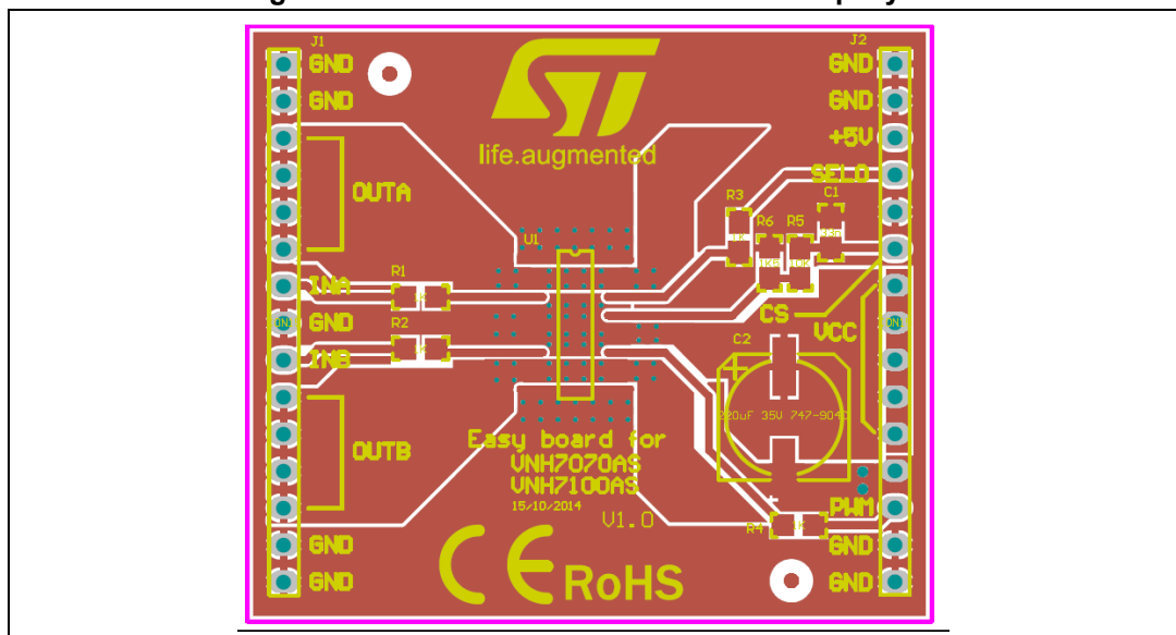
Figure 2. VN7070BAS evaluation board top layout
