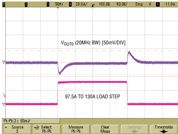
Figure 6. Output Voltage V_{OUT0} vs Load Current ( V_{OUT0} RANGE = 0)
