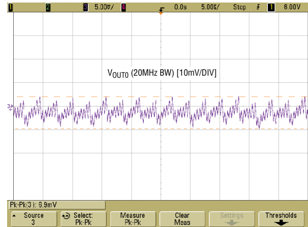
Figure 7. Output Voltage Ripple at V_{IN} = 12V , V_{OUT0} = 1V , I_{OUT0} = 130A
