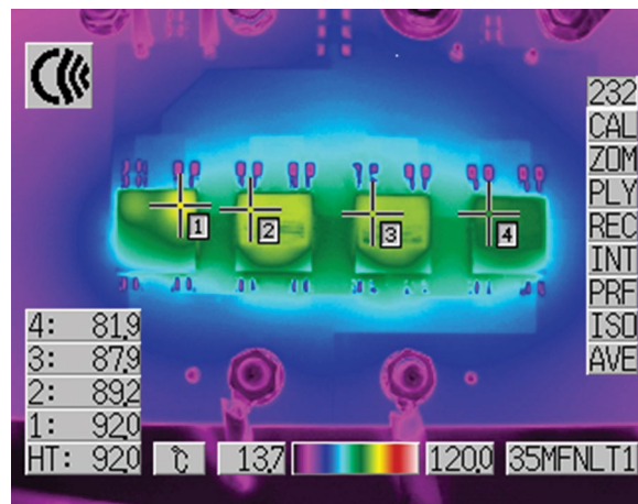
Figure 8. Thermal Performance at V_{IN} = 12V , V_{OUT0} = 1V , I_{OUT0} = 130A , T_A = 23.3^\circ C , Air Flow 300LFM
