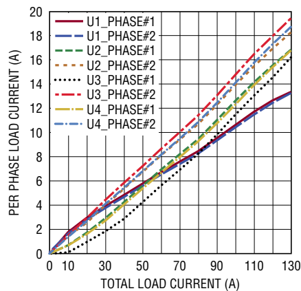
Figure 9. Current Sharing Performance at V_{IN} = 12V , V_{OUT0} = 1V
