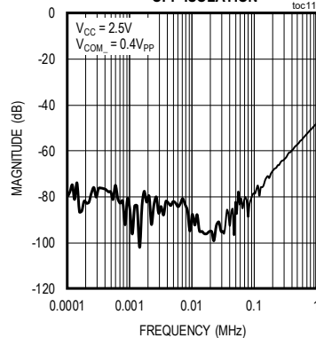
OFF-ISOLATION
