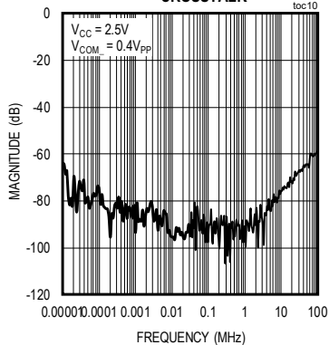
CROSSTALK
