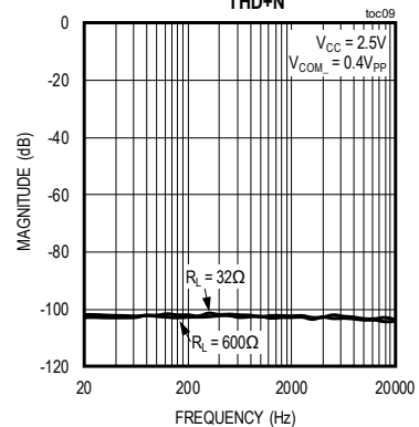
THD+N
