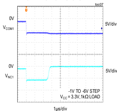
NEGATIVE OVLO RESPONSE TIME
