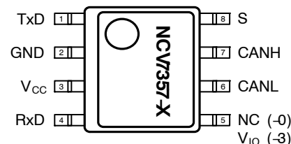
NCV7357MWx (Top View)
