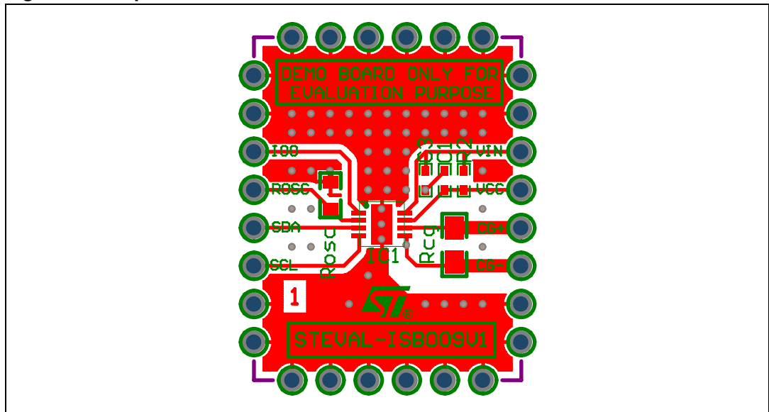
Figure 4. Top view of demonstration board
