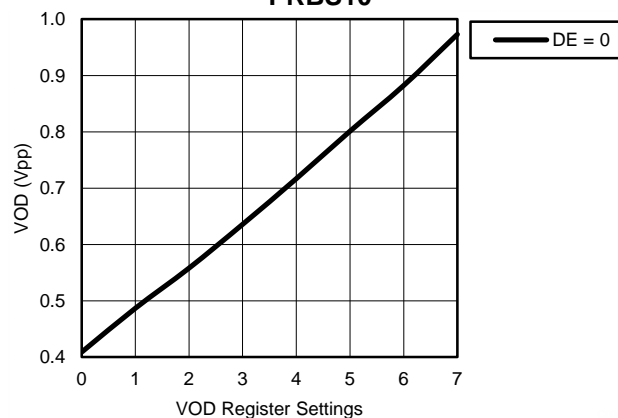
Figure 6. VOD vs. VOD and DEM Register Settings
