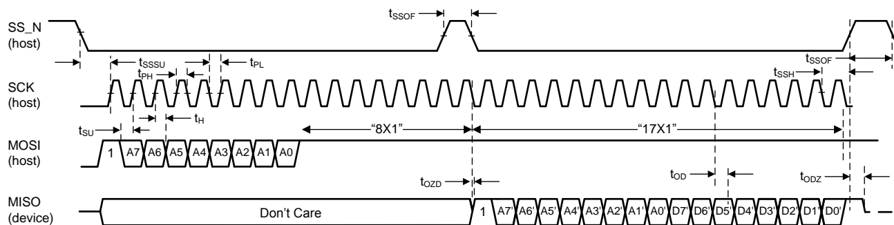
Figure 2. SPI Timing Parameters
