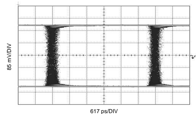
Figure 3. 2.97 Gbps, Input: 150 m Belden 1694A PRBS10
