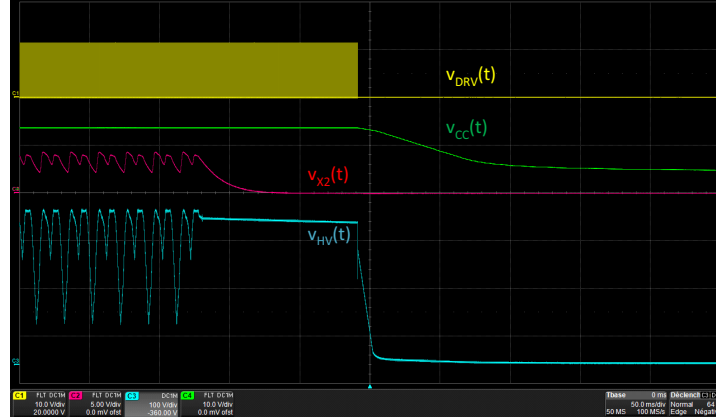
Figure 17. X2 Capacitor Discharge Function
