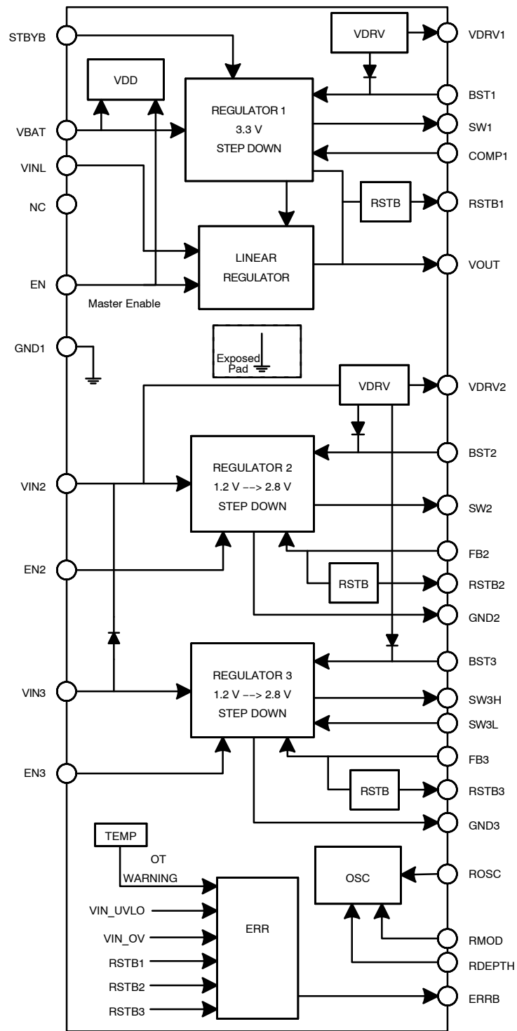
Figure 1. NCV97310 Block Diagram
