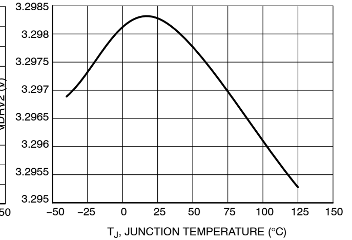
Figure 20. VDRV2 Voltage vs. Junction Temperature
