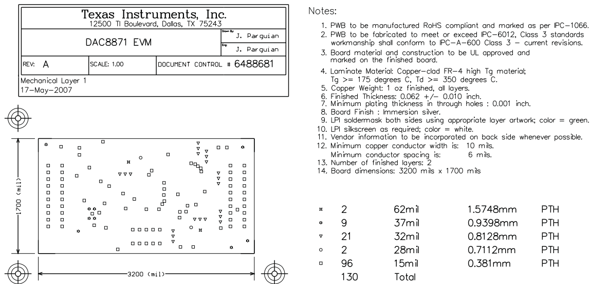
Figure 6. Drill Drawing
