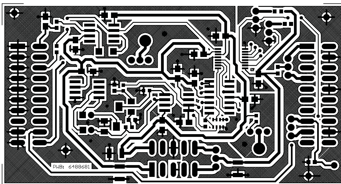
Figure 3. Layer 1, Top Signal Plane
