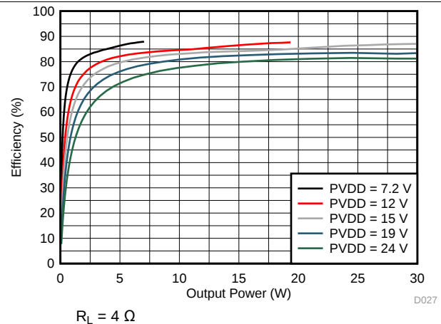
Figure 30. Efficiency vs Output Power
