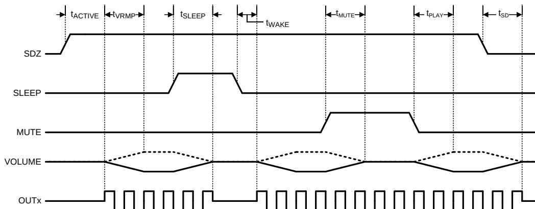
Figure 4. Mode Timing
