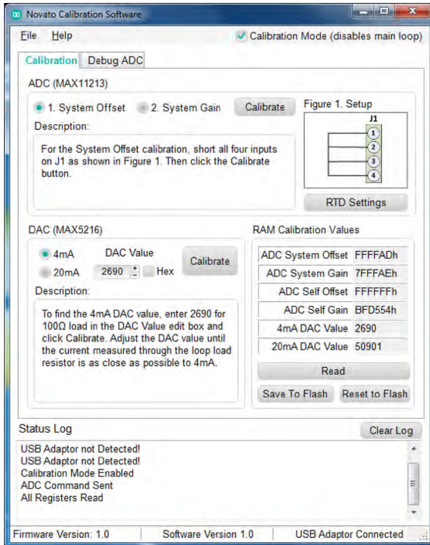
Figure 5. Novato calibration GUI.
