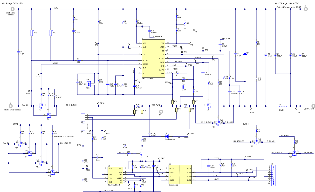
Figure 3. TPS23523EVM-863 Schematic
