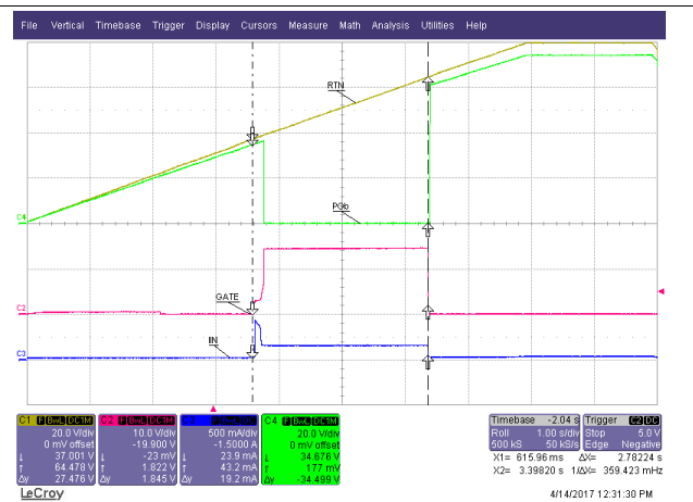
Figure 31. Plug in V_{IN,A} Backwards
