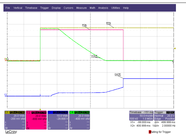
Figure 5. Start Up ( V_{IN} = 54\text{ V} )
