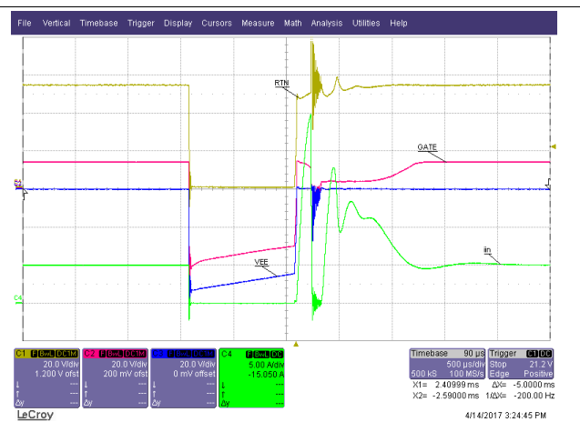
Figure 43. Load Step Into Overcurrent
