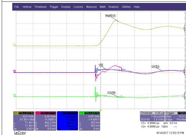
Figure 30. Unplug V_{IN,A}
