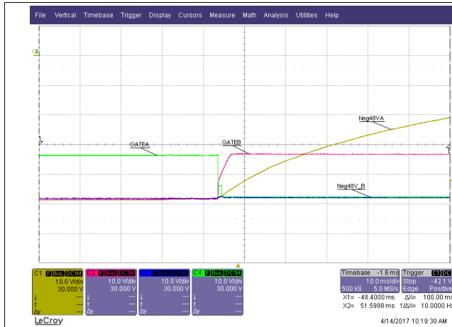
Figure 30. Unplug V_{IN,A}
