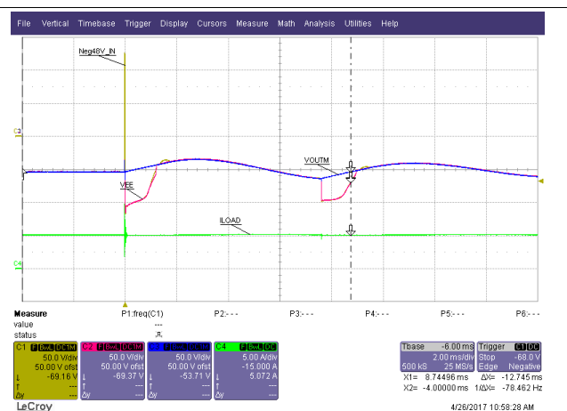
Figure 33. Undervoltage and Overvoltage (Rising)
