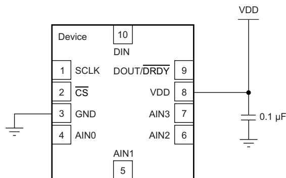
Figure 48. Power-Supply Decoupling
