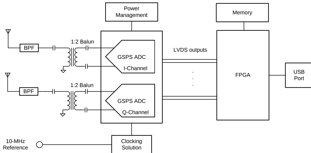
Figure 6-7. Simplified Schematic
