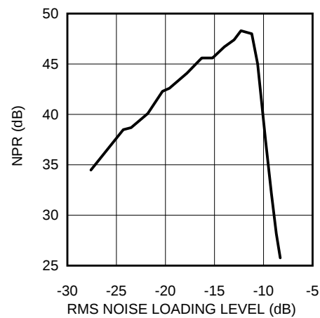
Figure 4-35. NPR vs. RMS Noise Loading Level (ADC12D1800)
