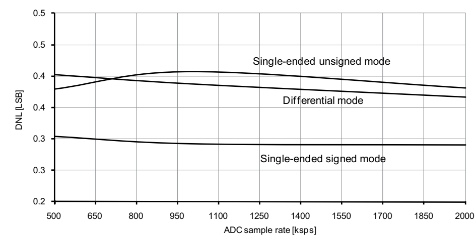
Figure 37-39. DNL error vs. sample rate. T = 25^{\circ}\text{C} , V_{CC} = 2.7\text{V} , V_{REF} = 1.0\text{V external} .
