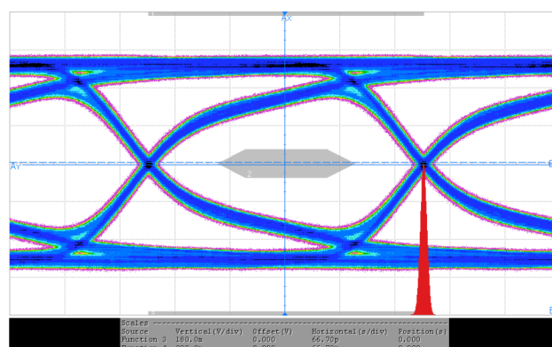
Figure 30. Eye at TP3 (output of TMDS461) with 3 m, 28 AWG HDMI cable, 3 Gbps Input TMDS data Rate, Slowest Rise and Fall Time Setting on TMDS outputs
