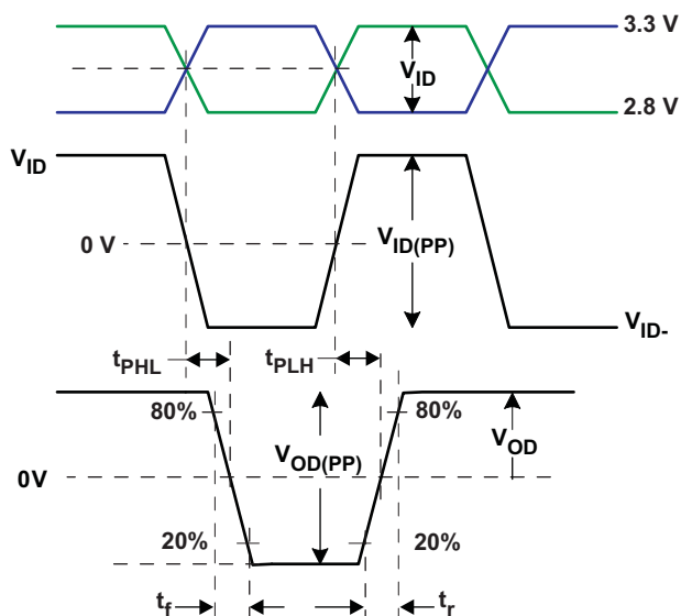
Figure 14. TMDS Main Link Timing Measurements
