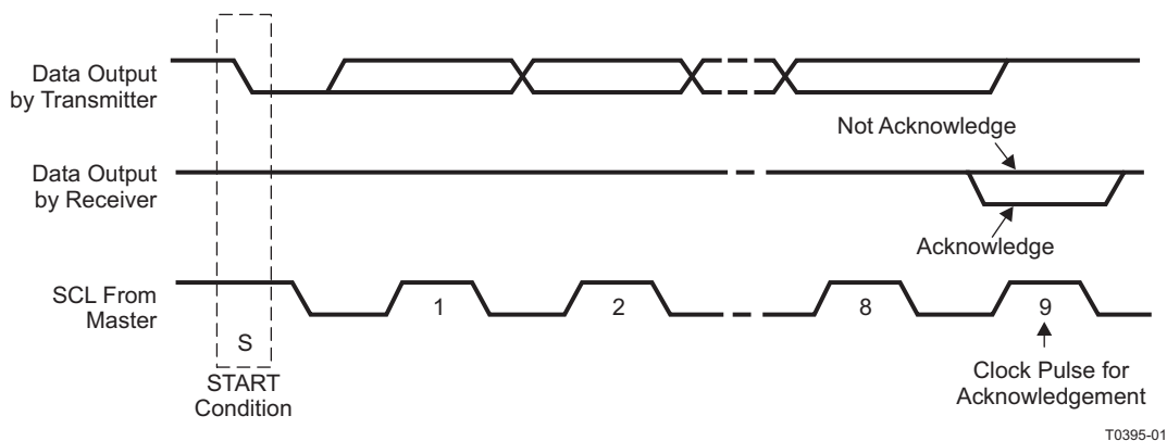
Figure 40. I²C Acknowledge
