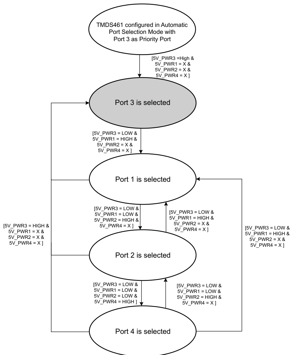
Figure 6. TMD5461 Configured in AutoSelect Mode, with Port 3 as Priority Port
