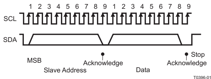
Figure 41. I²C Address, Data Cycle(s), and Stop
