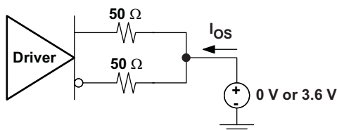
Figure 20. TMD5 Main Link Short Circuit Output Circuit
