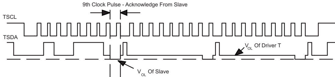
Figure 36. Bus T Waveform
