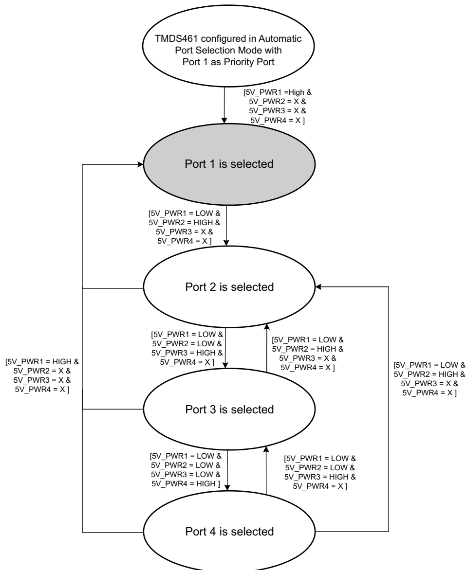
Figure 4. TMD5461 Configured in AutoSelect Mode, with Port 1 as Priority Port
