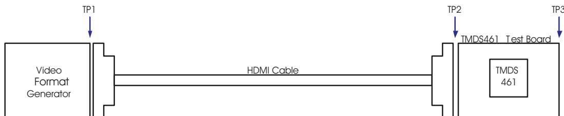
Figure 26. HDMI Cable Test-Point Configuration
