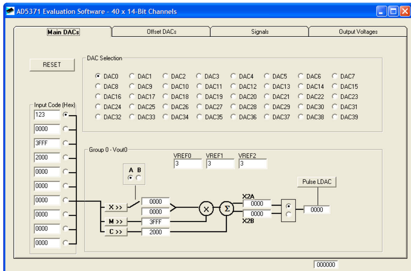
Figure 2. AD537x Tab 1 Software Screenshot
