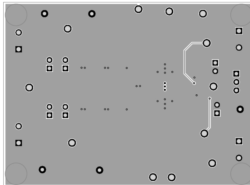
Figure 3. TPS22968NEVM Bottom
