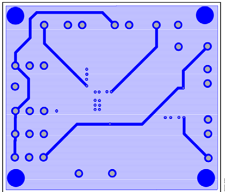
Figure 5. Second Layer
