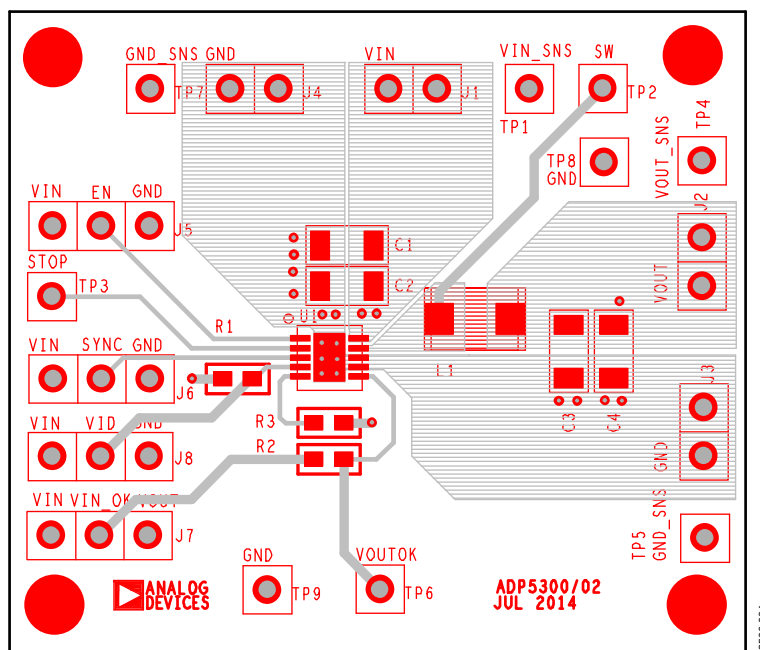
Figure 4. Top Layer
