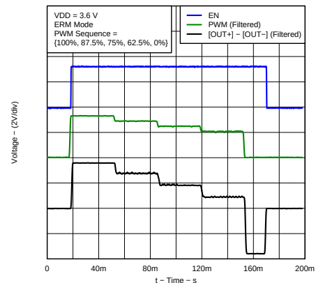
Figure 18. ERM PWM Modulation
