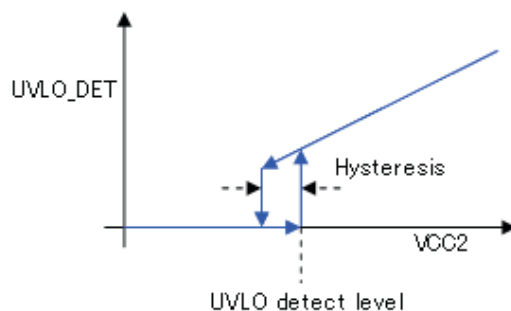
Figure 3. UVLO Hysteresis
