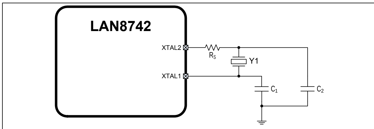
FIGURE 5-8: 100 \mu W 25 MHZ CRYSTAL CIRCUIT
