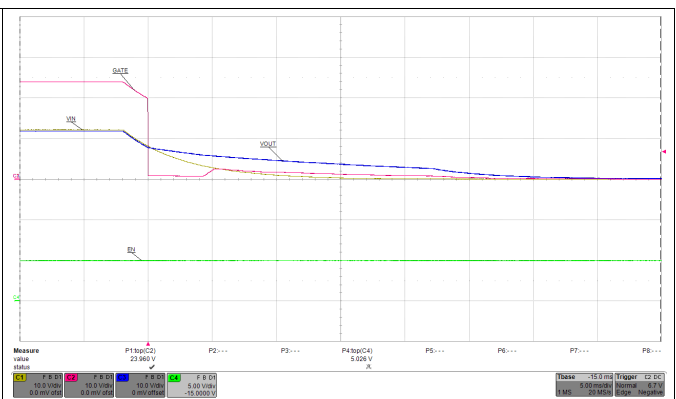
Figure 46. Shutdown
