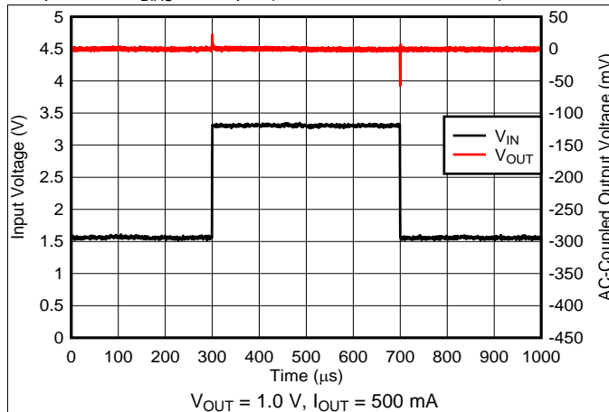
Figure 19. V_{IN} Transient
