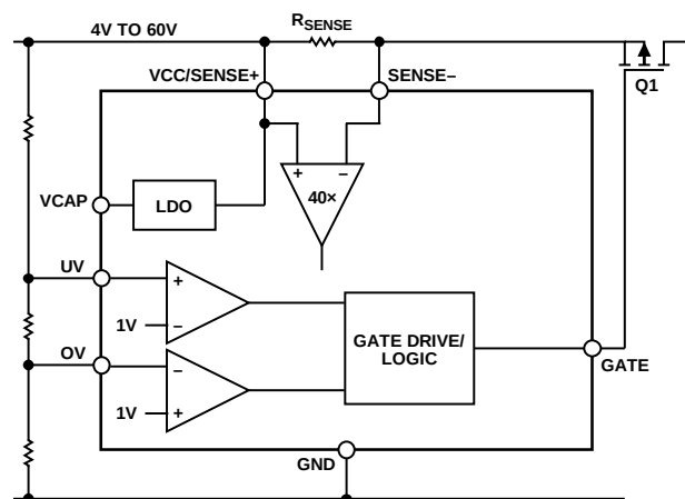
Figure 7. Undervoltage and Overvoltage Supply Monitoring
