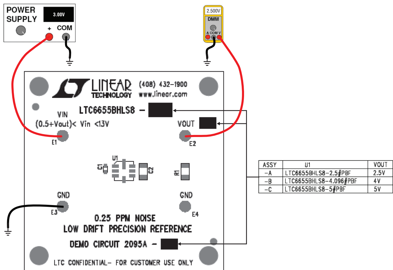
Figure 1. Test Setup
