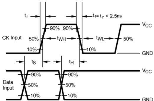
Figure 7. AC Waveforms
