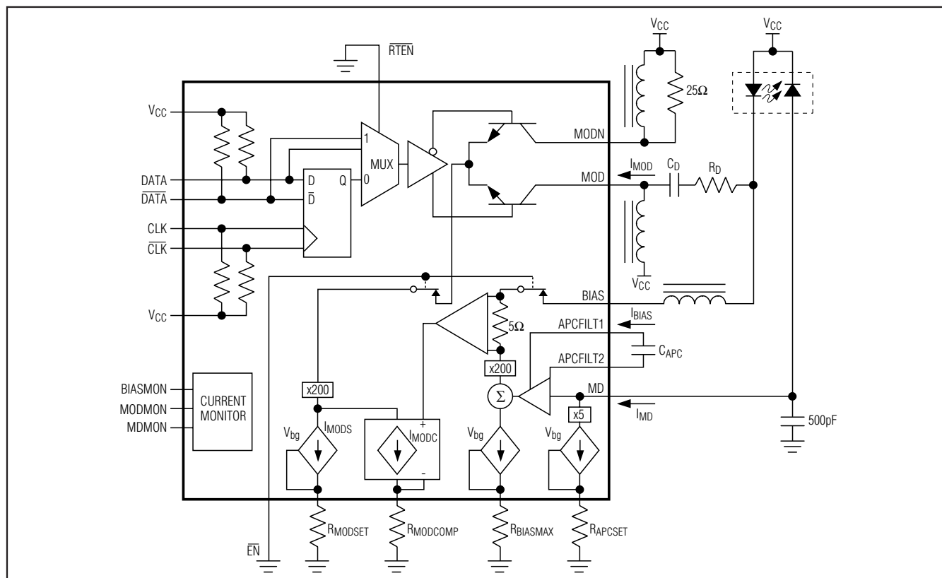
Figure 3. Functional Diagram
