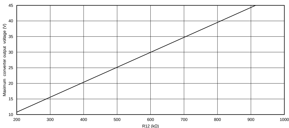
Figure 6. Converter Maximum Output Voltage vs R12
