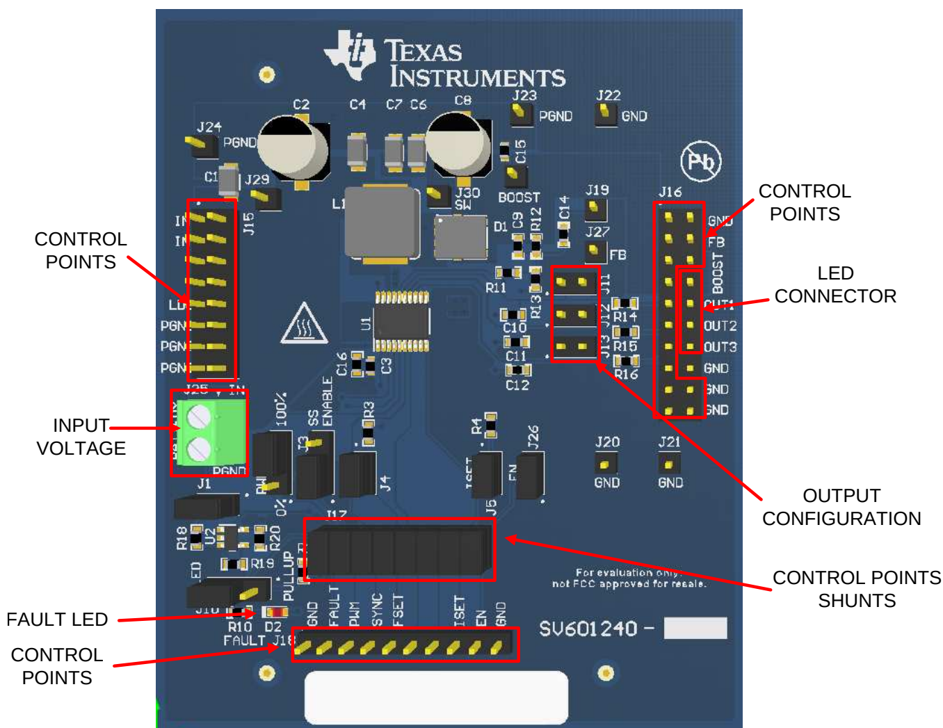
Figure 1. Evaluation Board Connectors and Setup
