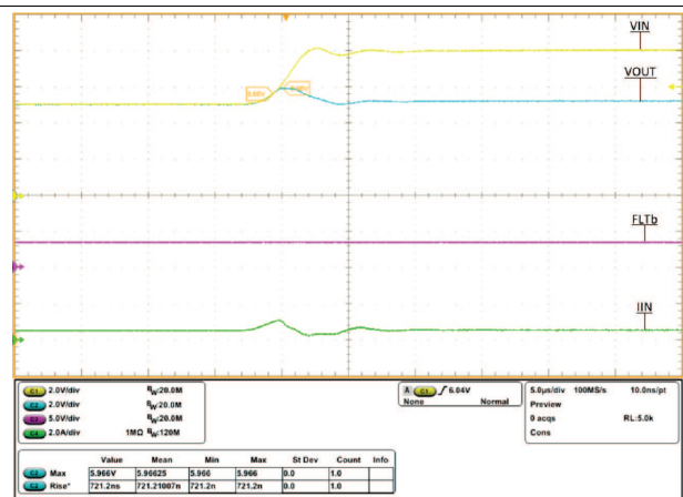
Figure 41. TPS259573 Overvoltage Lockout FLT Response
