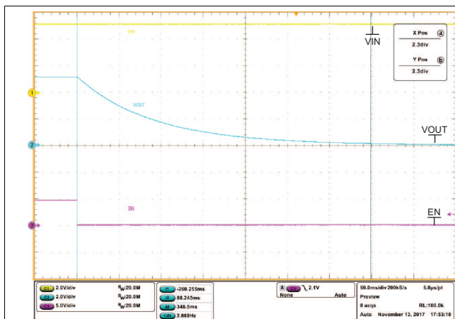
Figure 63. Output Voltage Discharge using TPS259535 without QOD [ V_{IN} = 5\text{ V} , EN = H \rightarrow L , C_{OUT} = 100\text{ }\mu\text{F} , R_{LOAD} = 1000\text{ }\Omega , R_{QODEXT} = \text{OPEN} ]
