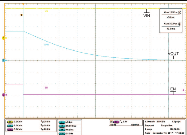
Figure 64. Output Voltage Discharge using TPS259535 with QOD [ V_{IN} = 5\text{ V} , EN = H \rightarrow L , C_{OUT} = 100\text{ }\mu\text{F} , R_{LOAD} = 1000\text{ }\Omega , R_{QODEXT} = \text{Short} ]
