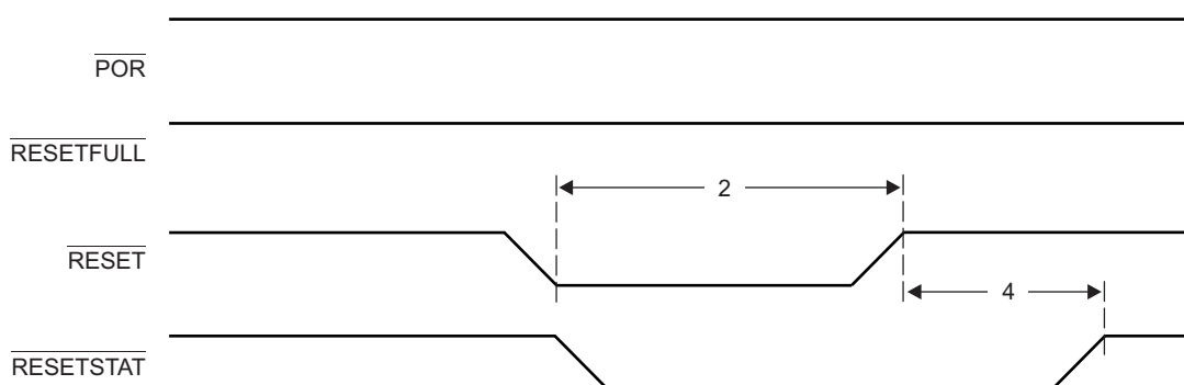
Figure 5-3. Soft/Hard-Reset Timing
