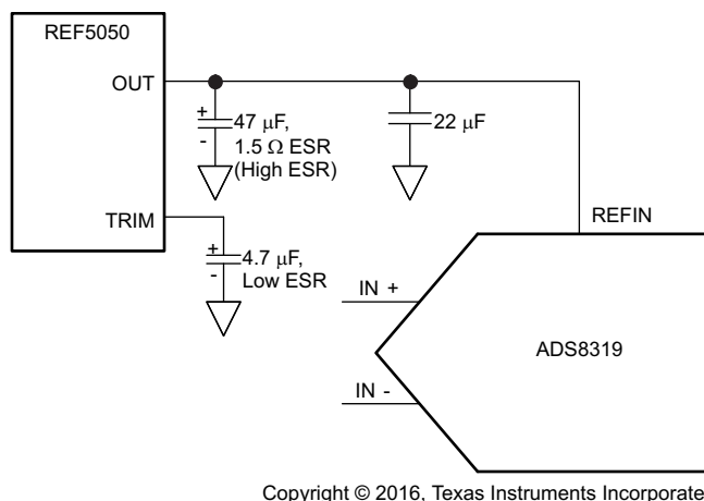
Figure 48. Direct External Reference Driving Circuit
