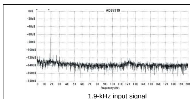
Figure 62. FFT
