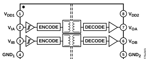
Figure 3. ADuM120N/ADuM225N Functional Block Diagram
