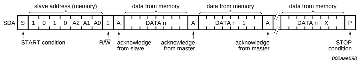
Fig 14. Sequential read
