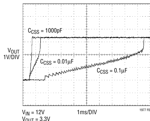
Figure 4. V_{OUT} dV/dt
