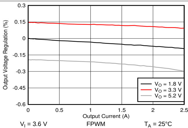
Figure 34. Load Regulation
