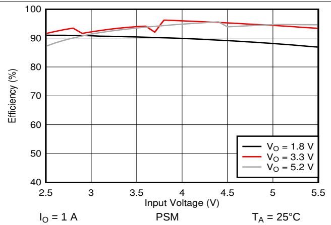
Figure 33. Efficiency versus Input Voltage
