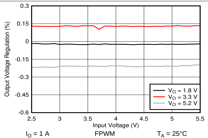
Figure 35. Line Regulation
