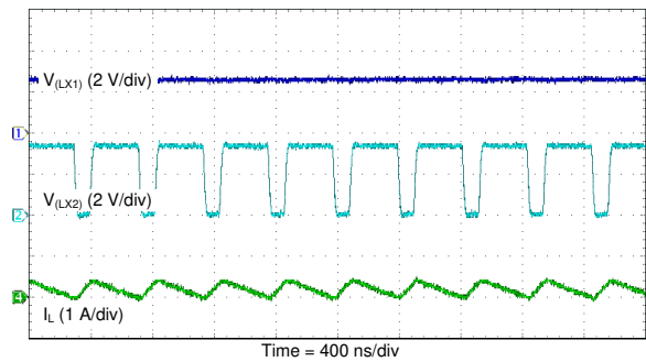
Figure 39. PWM Switching Waveforms (Buck Operation)
