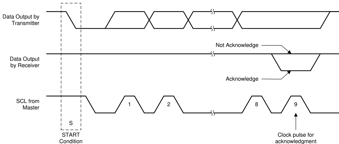
Figure 22. Acknowledge on the I²C Bus
