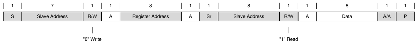
Figure 24. “Write” Data Transfer Format in Standard, Fast, and Fast-Plus Modes
