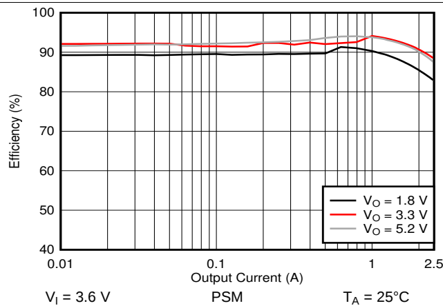
Figure 32. Efficiency versus Output Current
