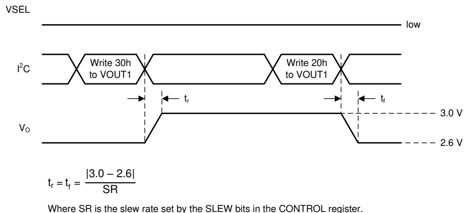
Figure 18. DVS Timing Using the I²C Interface
