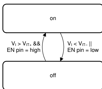
Figure 19. Device Functional Modes
