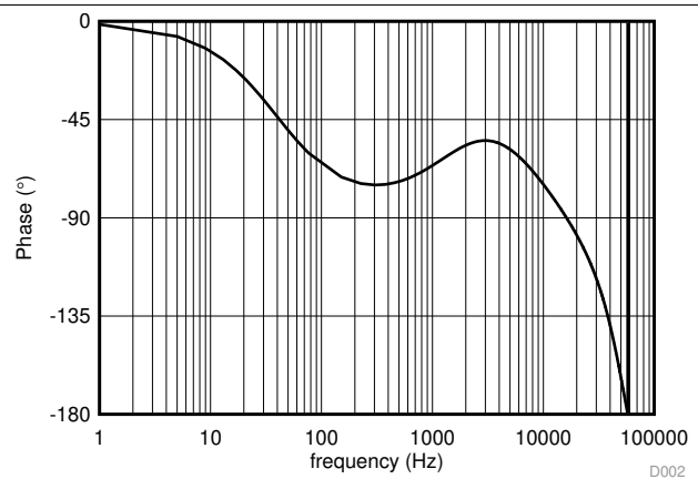
Figure 32. Converter Open-Loop Bode Plot - Phase
