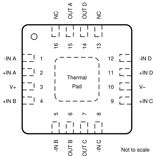
OPA4191 RUM Package 16-Pin WQFN With Exposed Thermal Pad Top View
